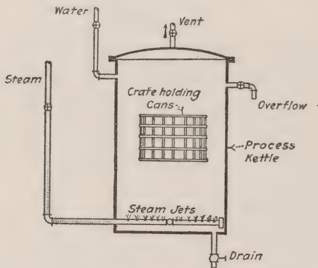
FIG. 9 PROCESS KETTLE
